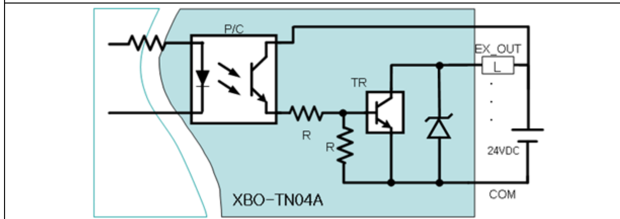
Circuit configuration
