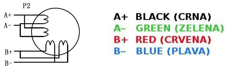
Figure 9: 8-lead motor parallel connections
