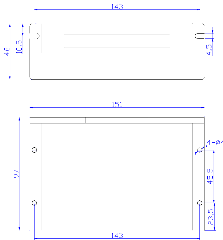
Figure 1: Mechanical specifications
